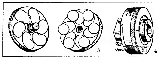
Fig. 3—Coupling plates with steel balls. Fig. 4—The complete coupling between armature shaft and motor, allowing automatic advancement of ignition by magnet
